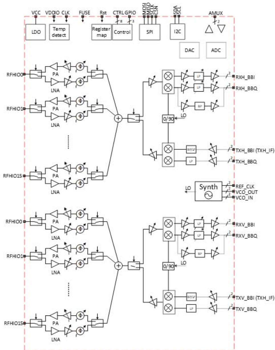
Figure 1. Block schematics TRB02801
